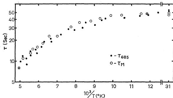
FIG. 6. A plot of the recovery half-life as a function of 1/T for the 685 mμ and M -band regions using crystals containing large \alpha_{M0}/\alpha_{F0} values.
