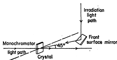
Fig. 1. Schematic arrangement of the crystal position relative to the measuring and irradiating beams.
